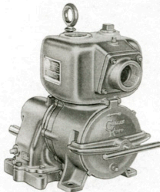
2" x 2" Model 12B2-G (above); also available in 3" x 3" Model 13A2-G.
